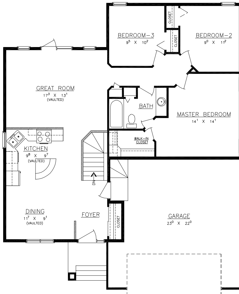
FLOOR PLAN
